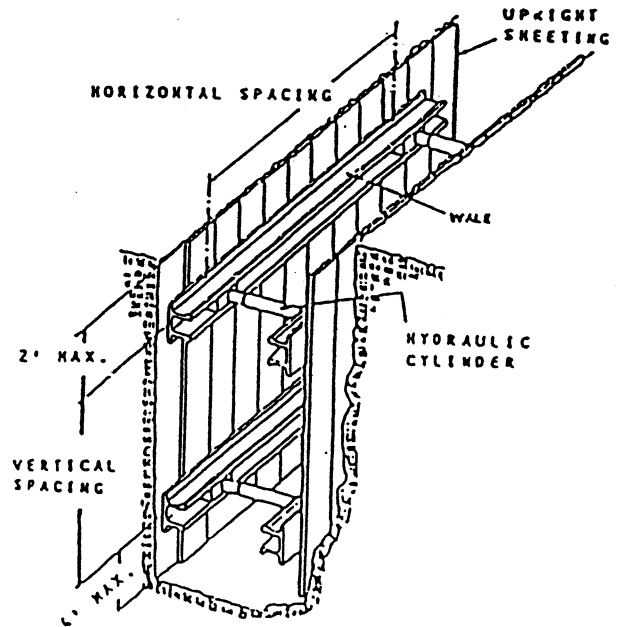
Figure No. 4 Aluminum hydraulic shoring - Waler System (typical)
