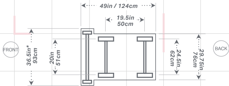
BOTTOM VIEW
